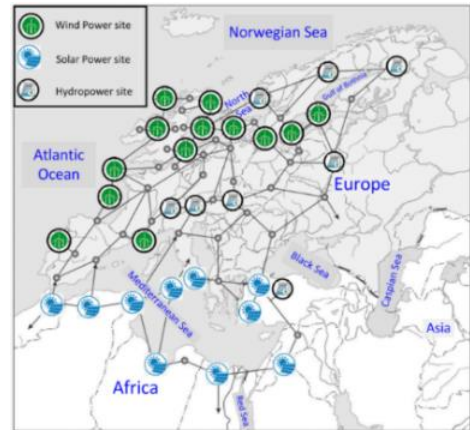
Figure 37: A conceptual plan of a European supergrid linking renewable energy projects
