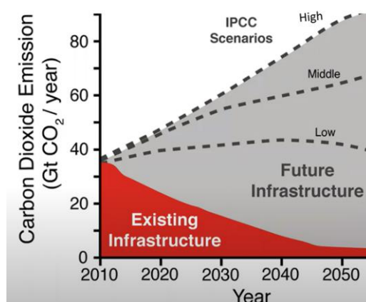
Figure 28: Future carbon dioxide emissions of infrastructures 99
